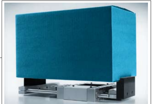
Pictured above is a special, dual-purpose LPG Gripper. The addition of a special rear toolbar provides "wide stance jaws (TFR)" for gripping the large carton shown. Standard "cantilevered jaws (TBF)" for smaller parts gripping can be seen beneath the carton to the left.
