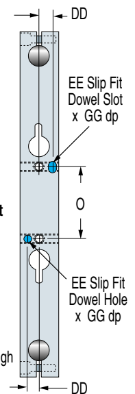
View D-D Toolbar Option D
